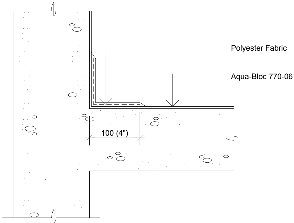
Monolithic Deck to Wall Juncture
