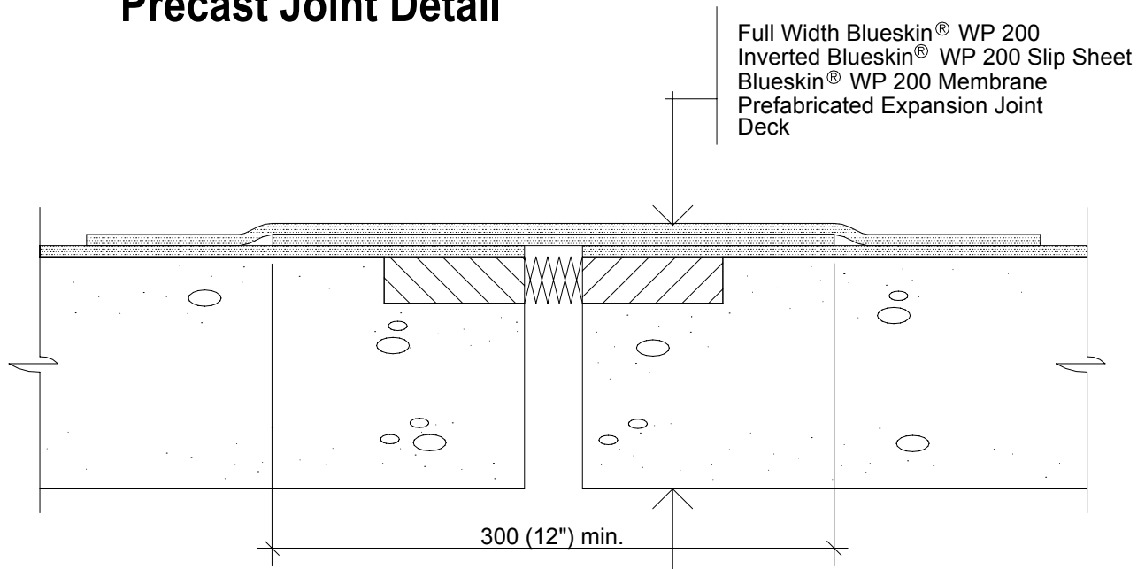
Expansion Joint
